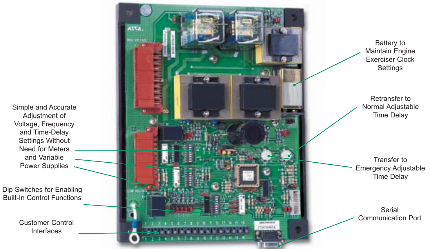
Fig. 9: Microprocessor Controller
