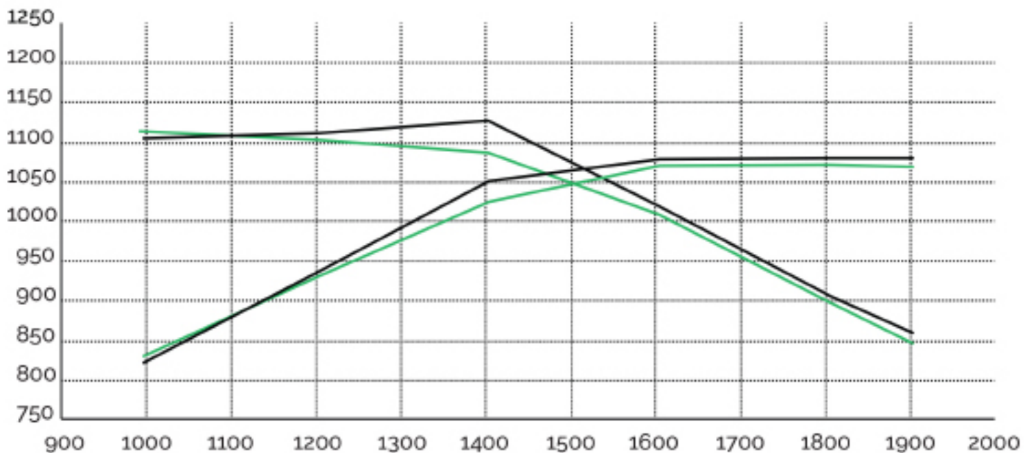
13L Power and Torque Pipeline NG and Commercial LPG
